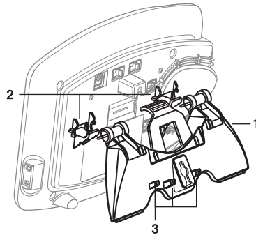
Figure 12 Attaching the Support Bracket
